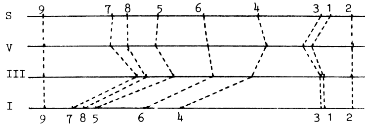
Figure 6. Utility scales from table 5.
