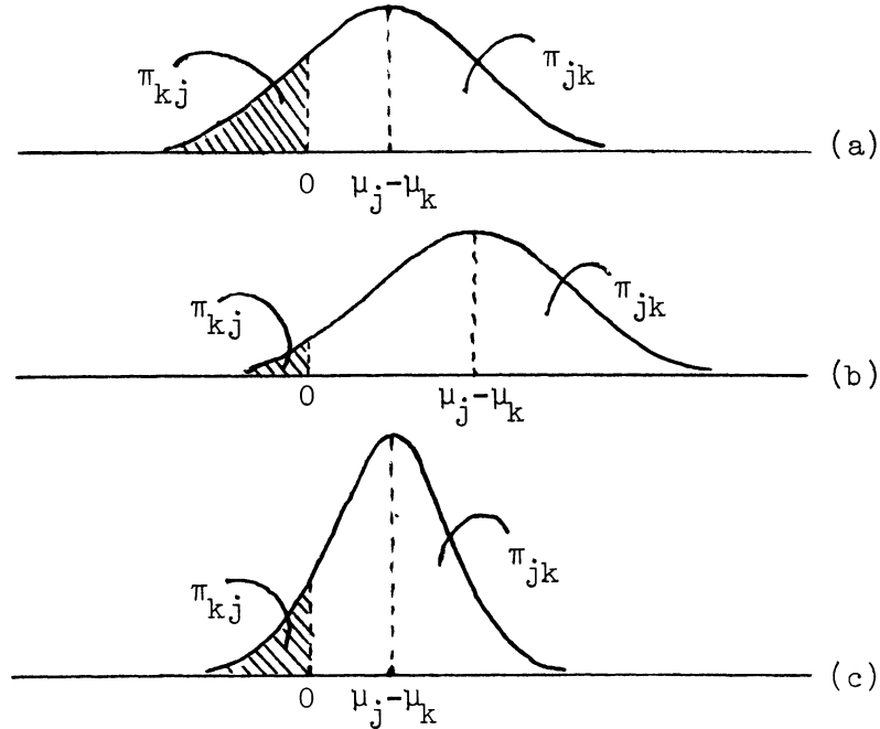
Figure 3. Three distributions of utility differences.
