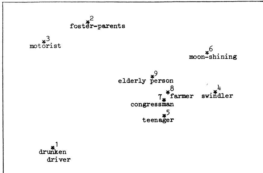
Figure 7. Cognitive map obtained from the immorality judgments in table 5 ( L(X,u) = 0.0511 ).
