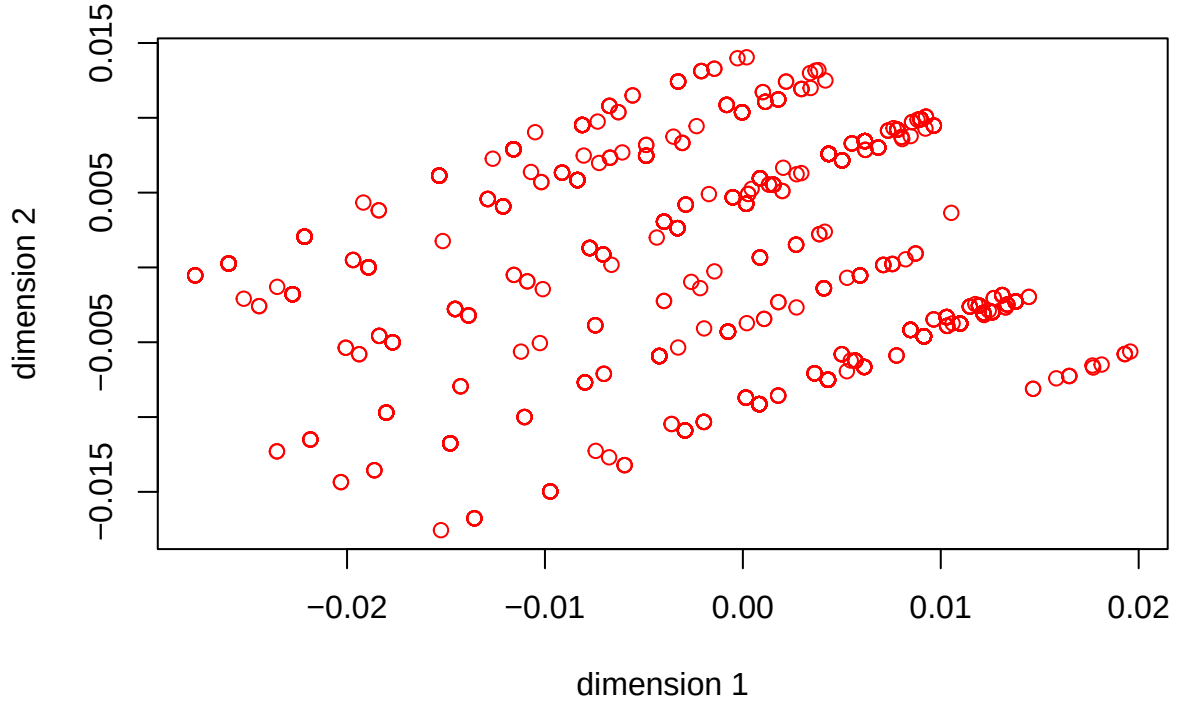
Figure 12: PRIMALS GALO Object Scores
