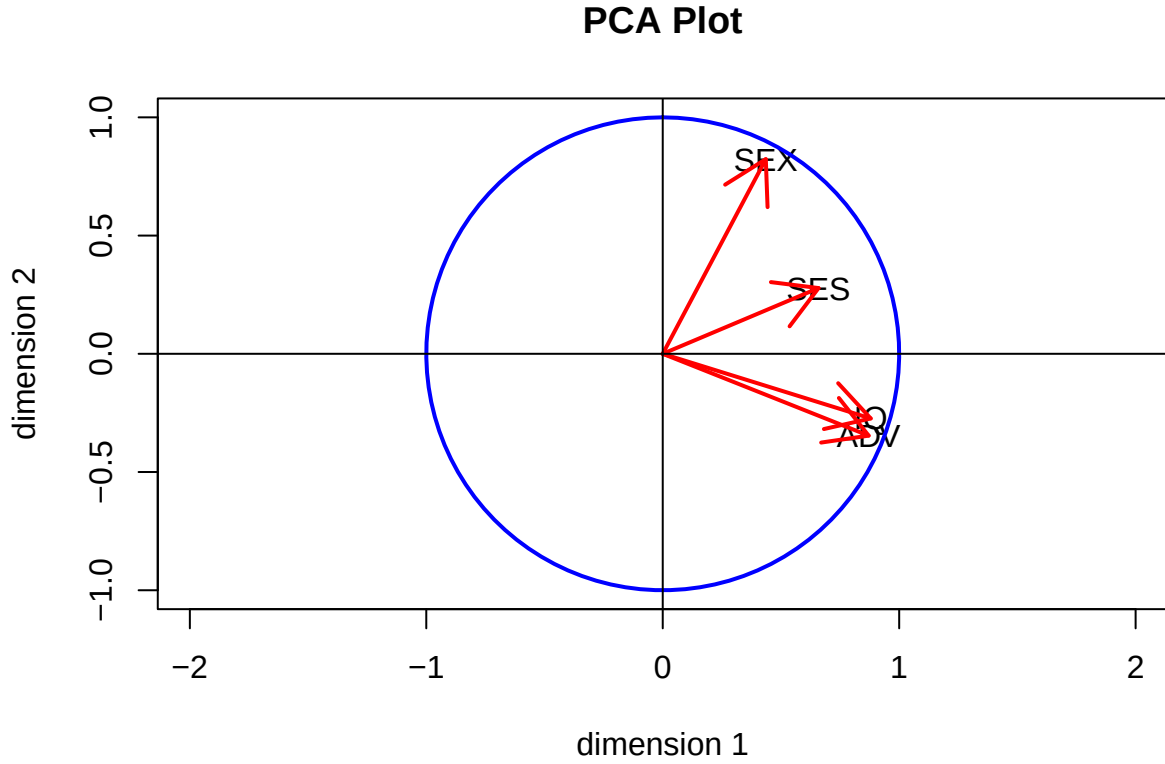
Figure 10: PRIMALS GALO PCA Plot
