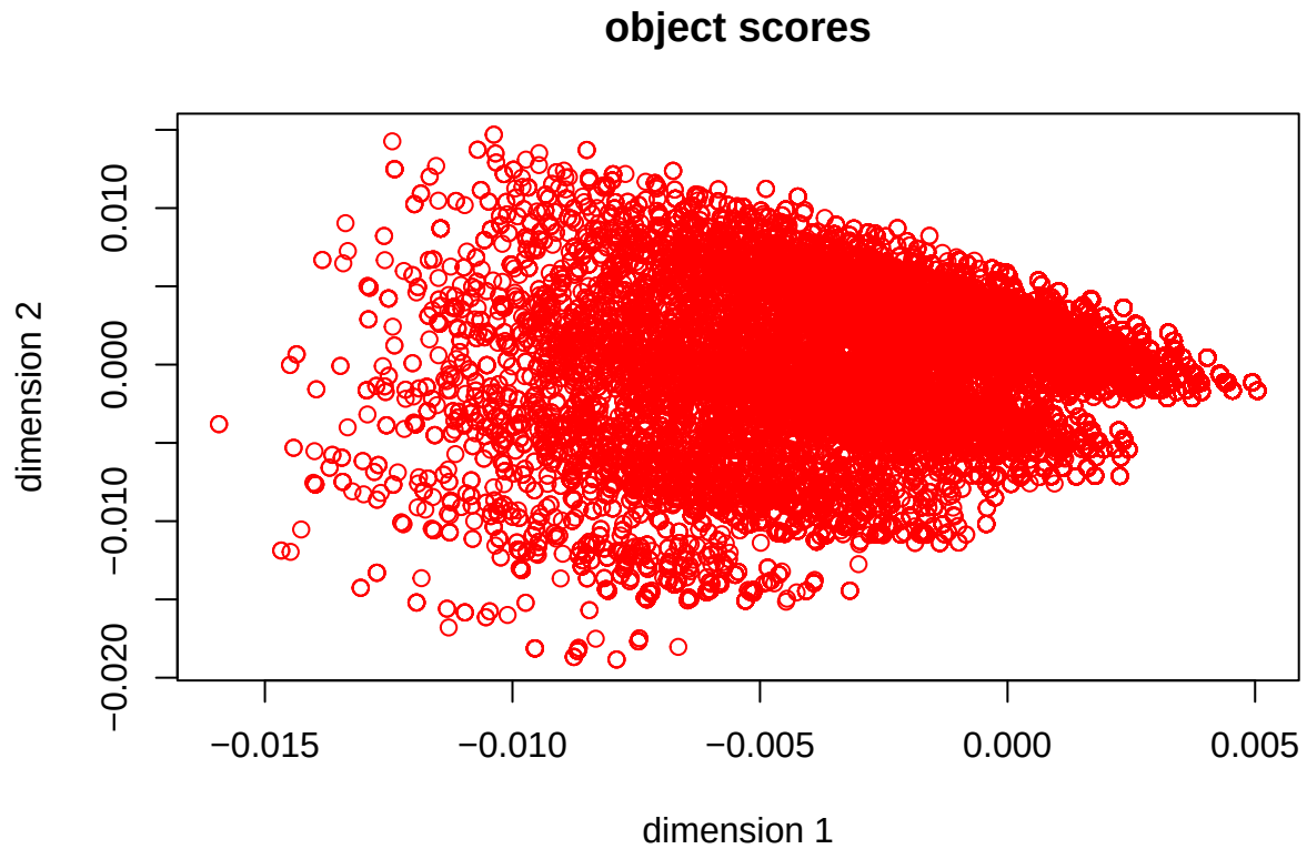
Figure 24: Norway Object Scores, Additive
