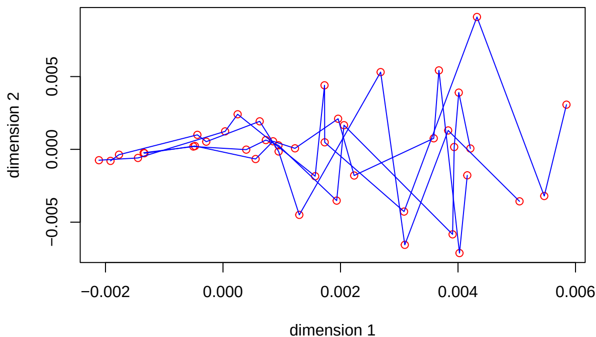
Figure 28: SBL Norway Category Quantifications, Different R
