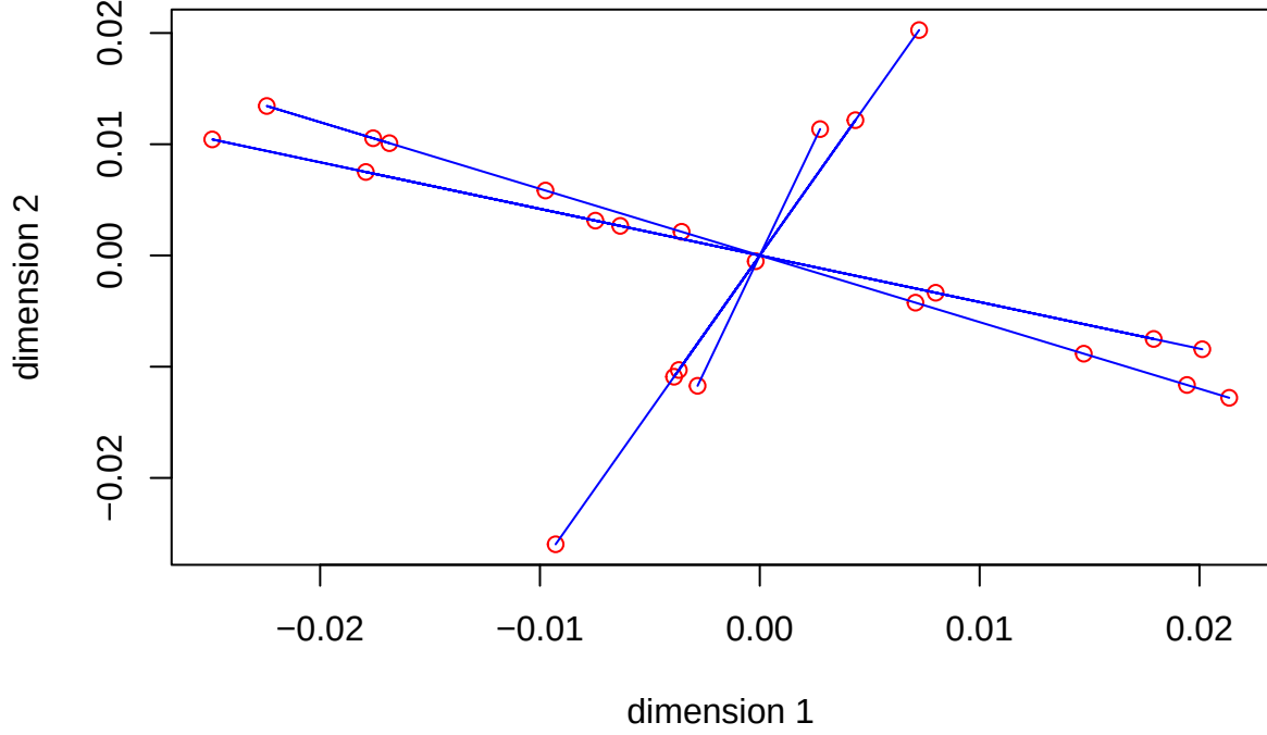
Figure 14: PRINCALS GALO Category Quantifications
