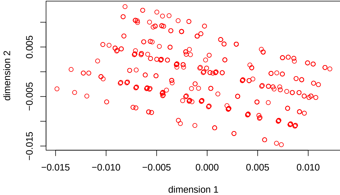
Figure 15: PRINCALS GALO Object Scores
