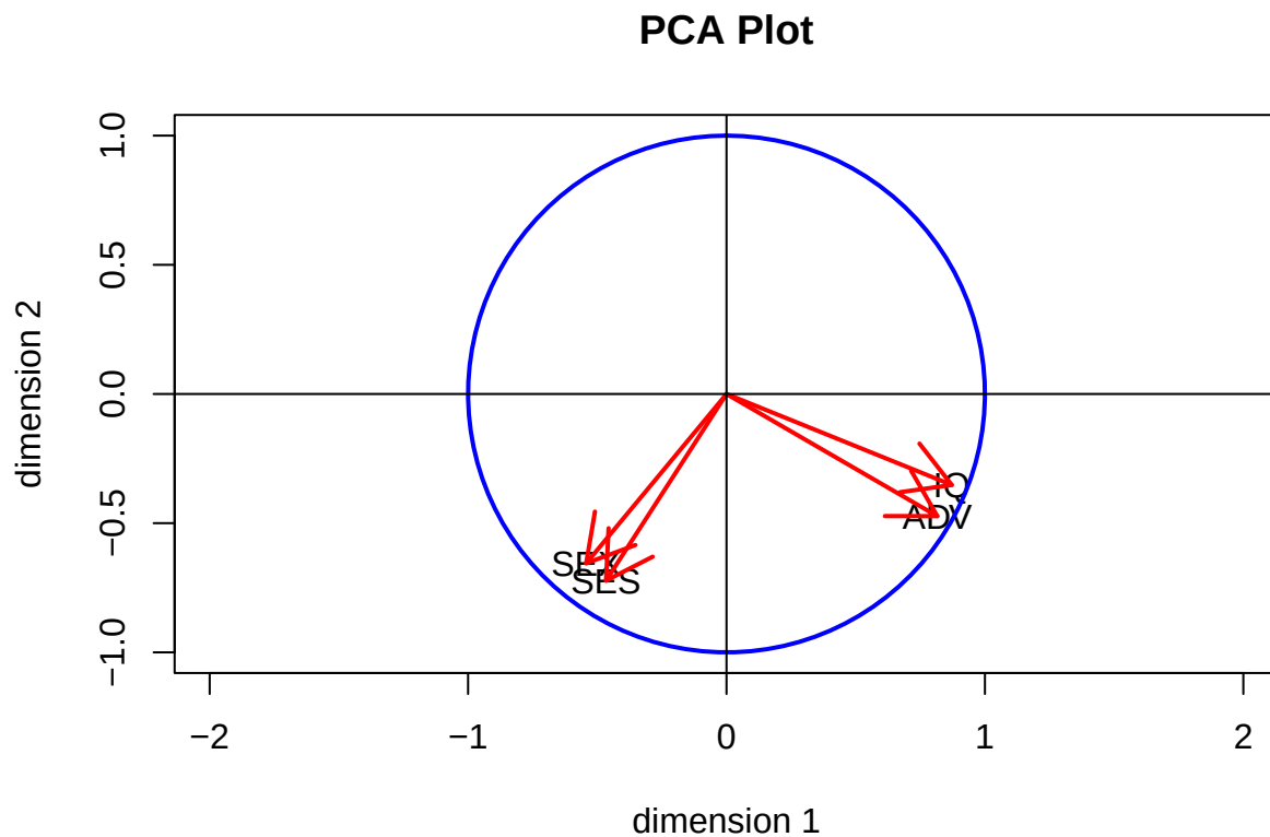
Figure 13: PRINCALS PCA Plot
