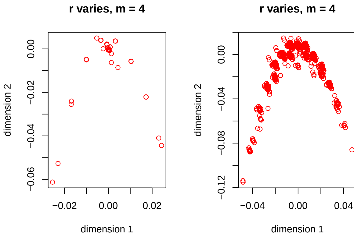
Figure 6: Normal Croissants, m = 4 , r is various
