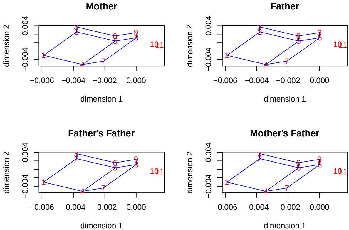
Figure 26: Norway Object Scores, Additive and Equality
