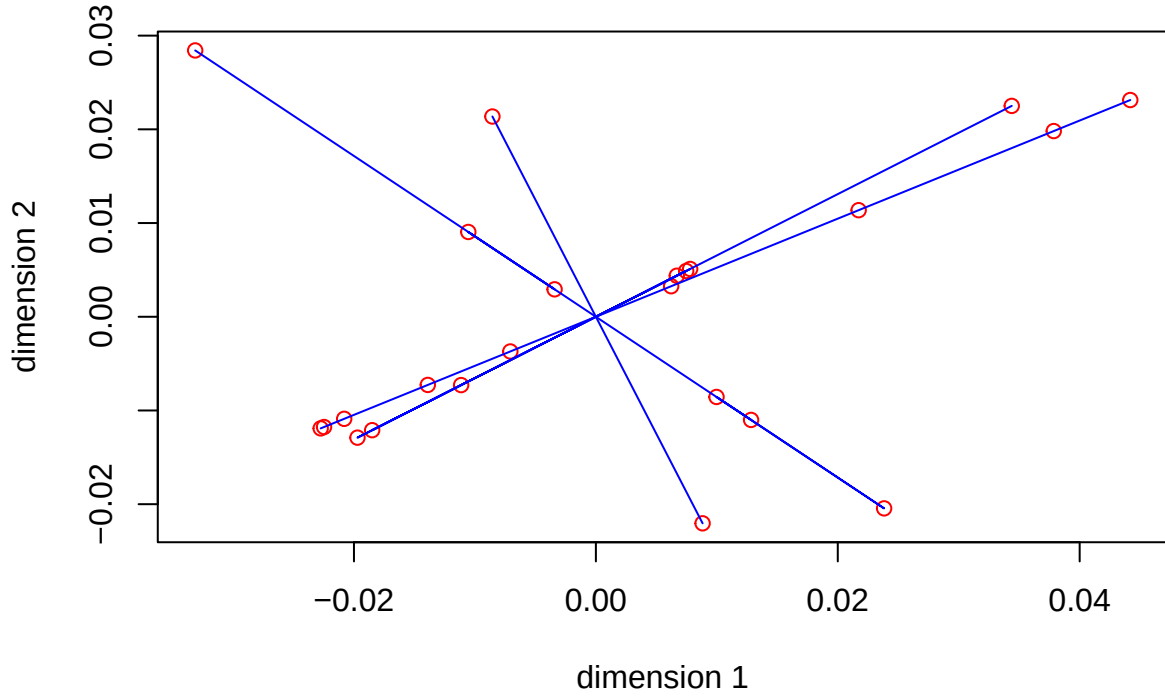
Figure 17: SBL GALO Category Quantifications, Same R
