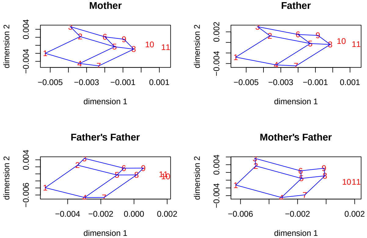
Figure 23: Norway Category Quantifications, Additive
