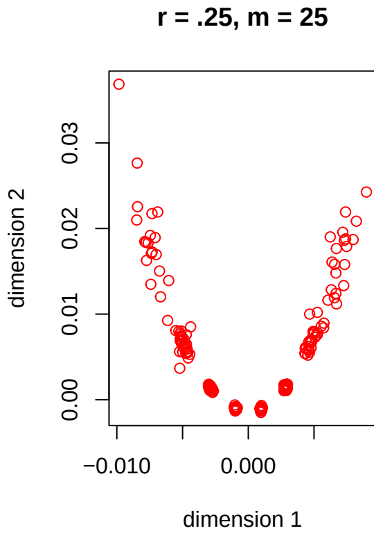
Figure 4: Normal Croissants, m = 25 , r = .25
