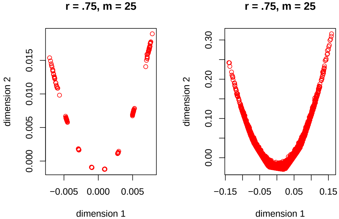
Figure 3: Normal Croissants, m = 25 , r = .75
