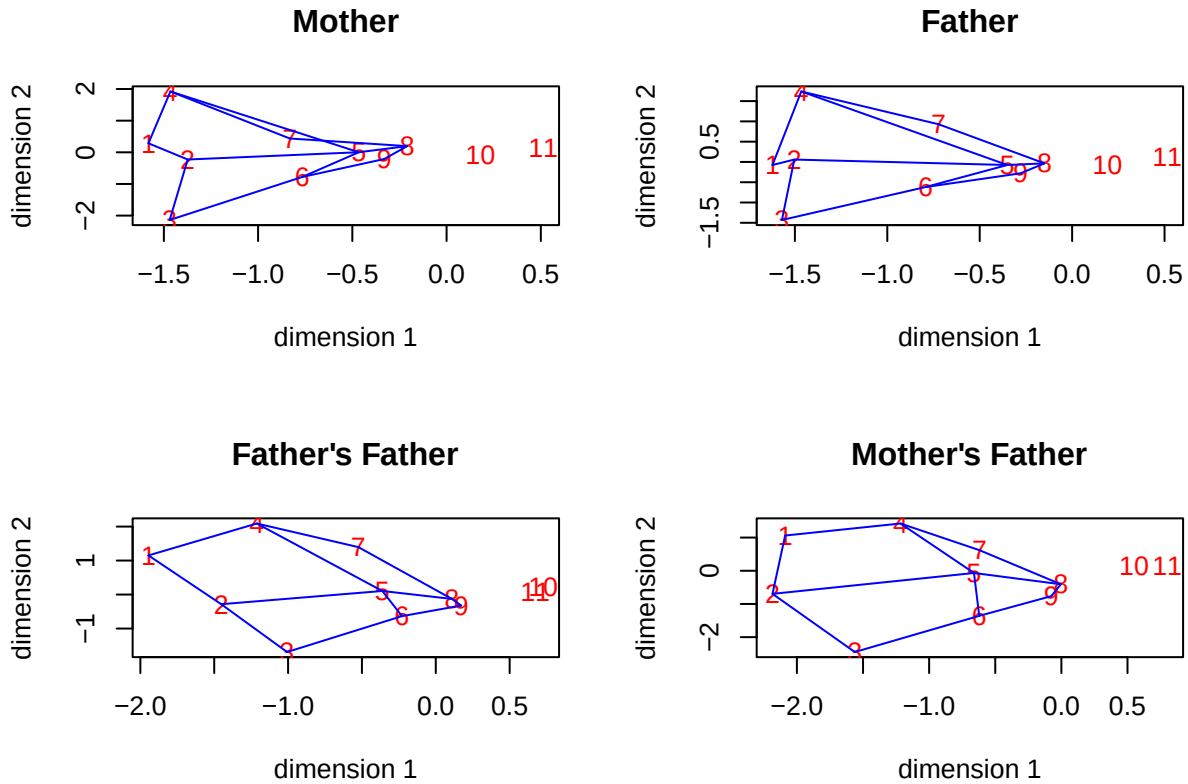
Figure 20: Norway Category Quantifications, Separate
